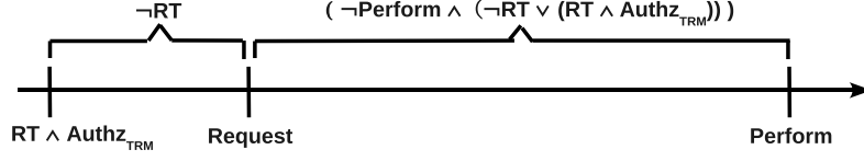
Figure 4.10: Formula \varphi_1 .
