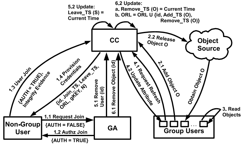
Figure 4.1: g-SIS Architecture.
